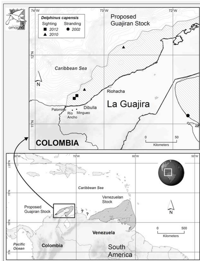
Figure 1. Long-beaked common dolphins ( Delphinus capensis ) in Colombian Caribbean waters. The upper map shows the locations of the four sightings made in 2010 and 2012 off the lower Guajira Peninsula, northern Colombia (solid triangles and squares, respectively). The location of the 2002 stranding in western Venezuela reported by Ramírez Carroz and González-Fernández (2004) is also plotted (solid circle). The lower map shows the Caribbean region with schematic polygons (hatched areas) illustrating the distribution of the putative ‘Venezuelan Stock’ in the southeastern Caribbean proposed by Jefferson et al. (2009) and the distribution of the ‘Guajiran Stock’ tentatively proposed in this paper for the southwestern Caribbean. The delineation of the latter was based on oceanographic considerations and extends roughly from the coastline to the 200m isobath. An alternative interpretation is a more-or-less continuous distribution for the species, extending from eastern Venezuela to northern Colombia, indicated by question marks.
